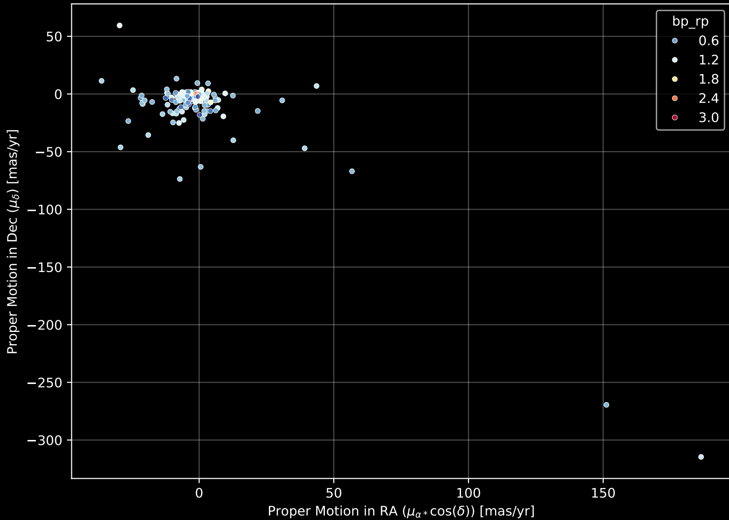
GALAH DR4 Field: [4501] Proper Motion Diagram (n= 163)
