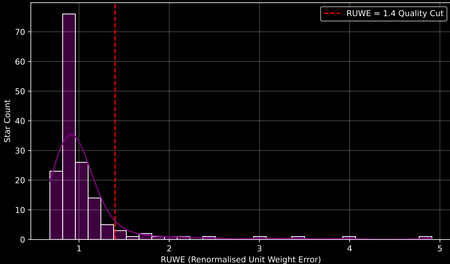
GALAH DR4 Field [4501] RUWE Distribution (n= 158)
