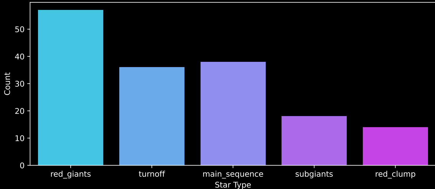
GALAH DR4 Field: [4501] Count plot of Star Type
