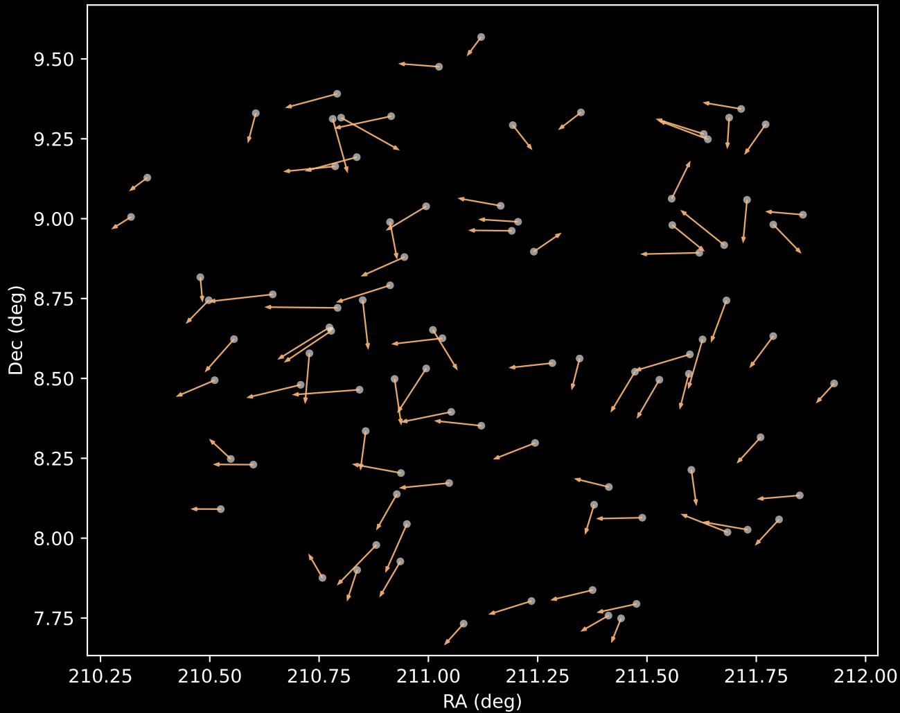
GALAH DR4 Cluster 3 Proper Motion Vectors (n=89)
